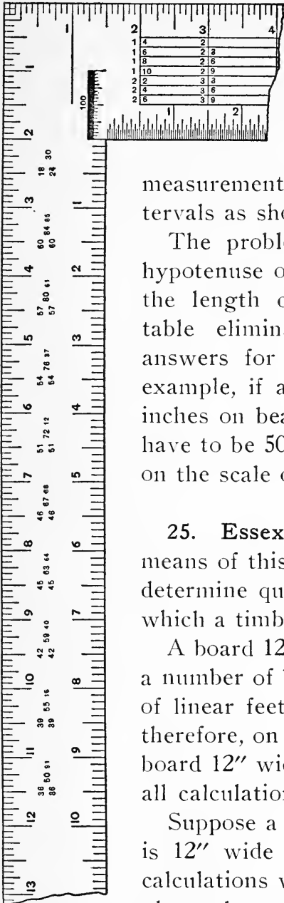
FIG. 26. BRACE MEASURE TABLE.
